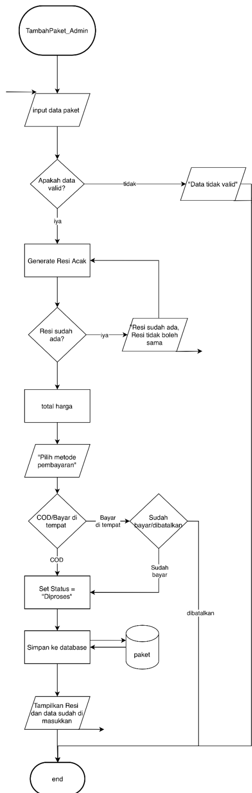
Gambar 13.1 Flowchart Tambah Paket Admin
