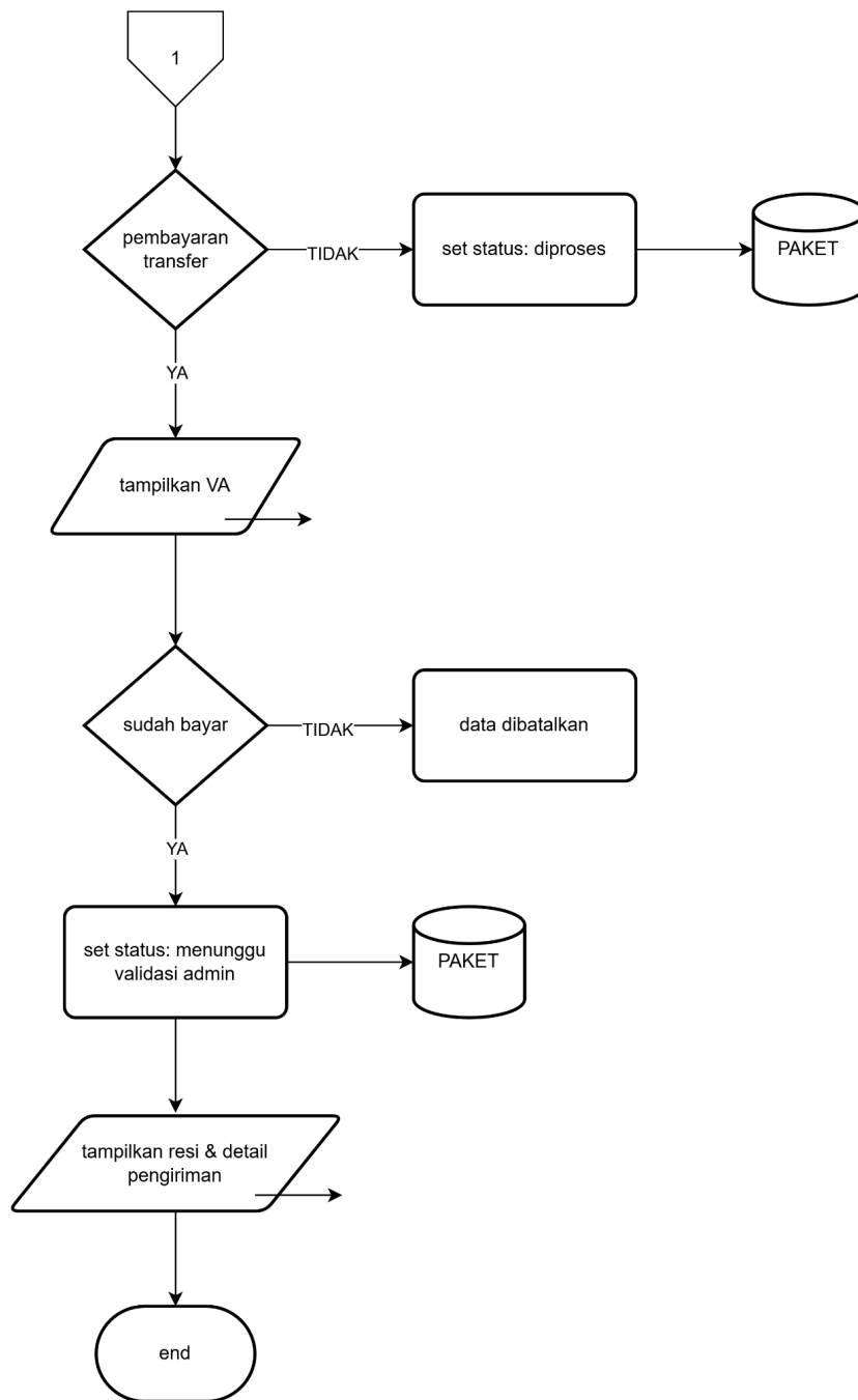
Gambar 6.2 Flowchart Tambah Paket User (2)
