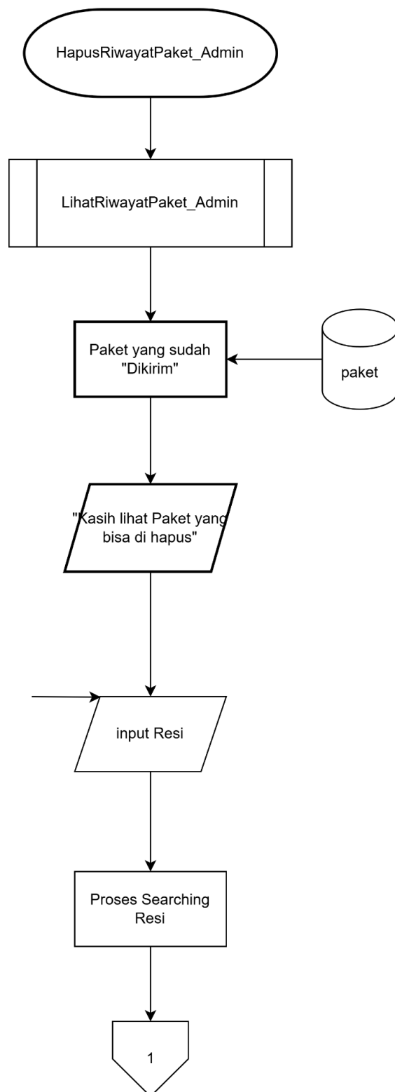
Gambar 16.1 Flowchart Hapus Riwayat Paket Admin (1)
