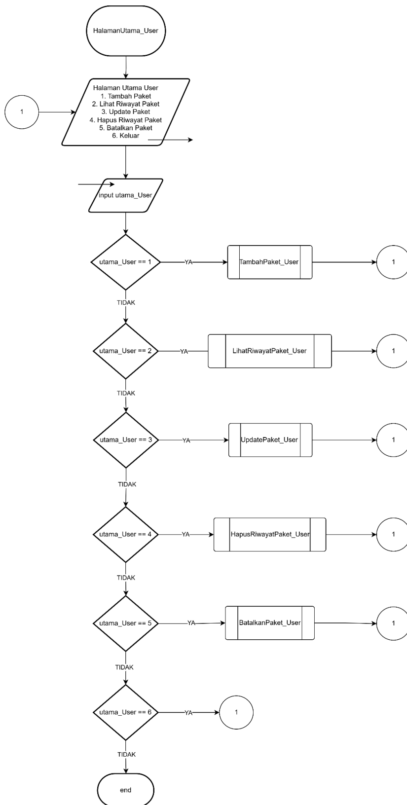
Gambar 5.1 Flowchart Halaman User
