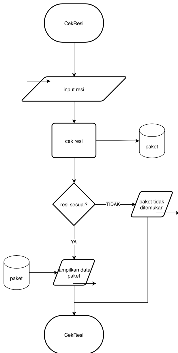
Gambar 18.1 Flowchart Cek Resi
