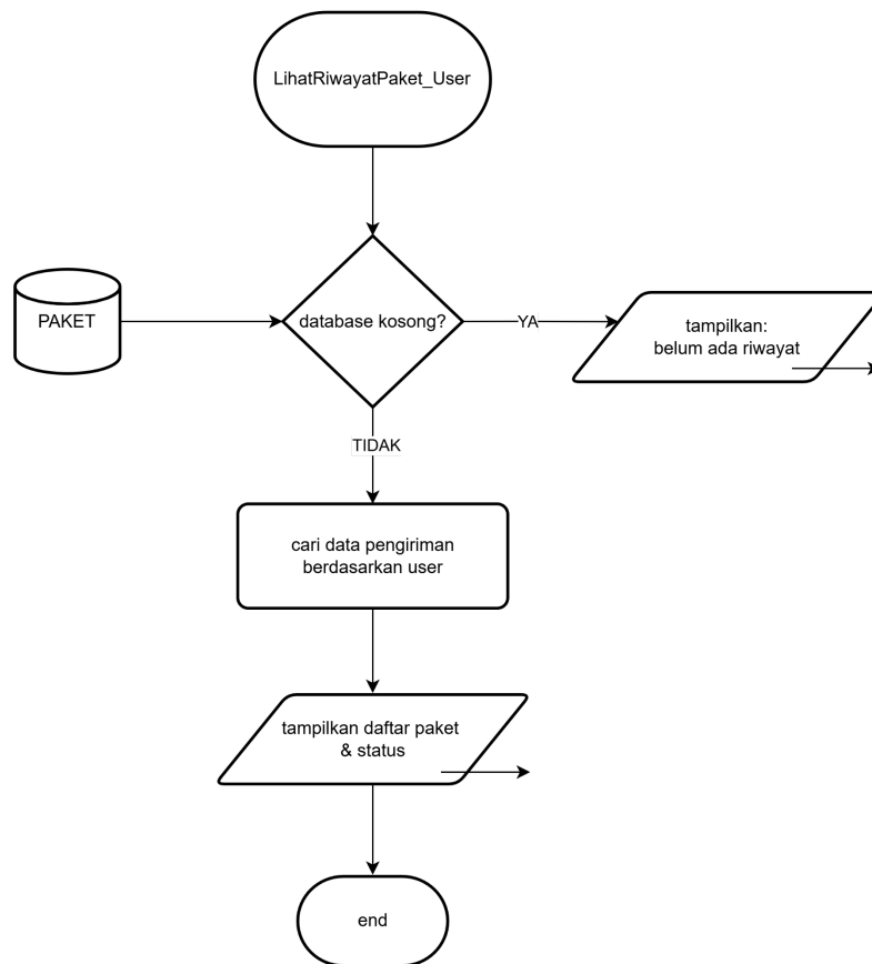
Gambar 7.1 Flowchart Lihat Riwayat Paket User
