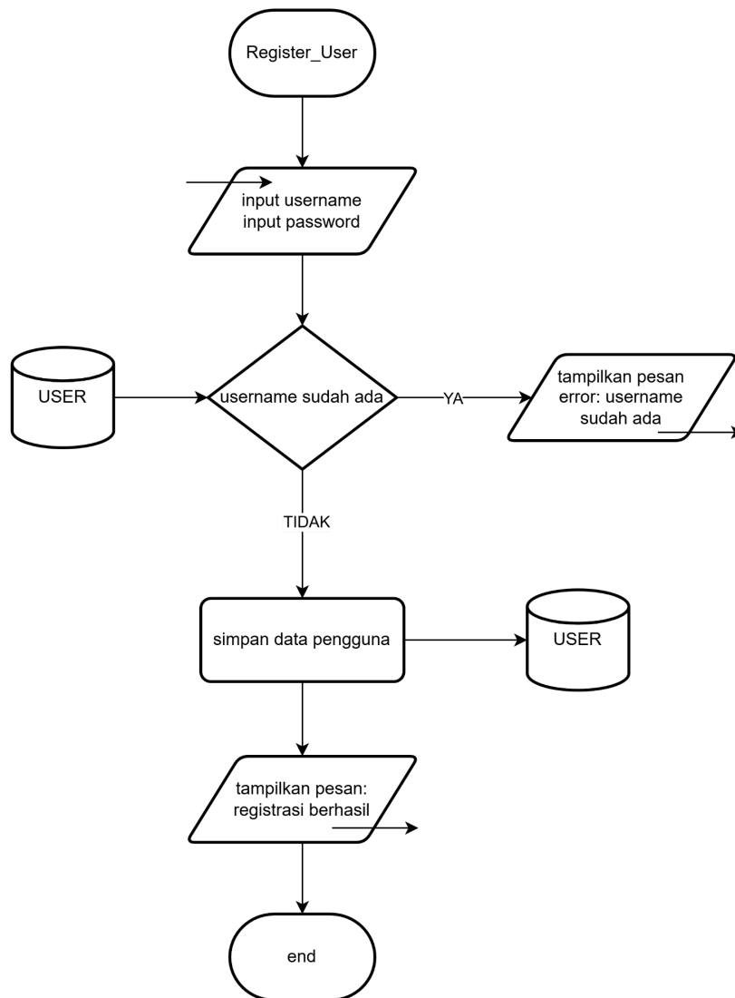
Gambar 3.1 Flowchart Register User
