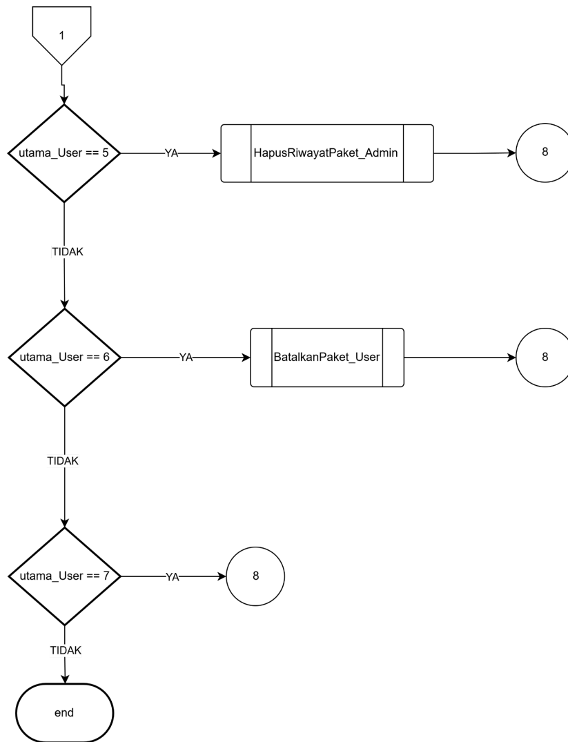
Gambar 12.1 Flowchart Halaman Utama Admin (2)
