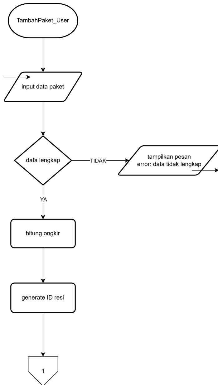
Gambar 6.1 Flowchart Tambah Paket User (1)
