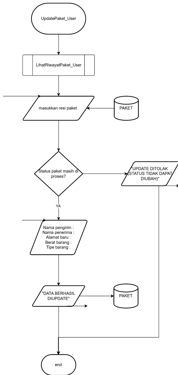
Gambar 8.1 Flowchart Update Paket User
