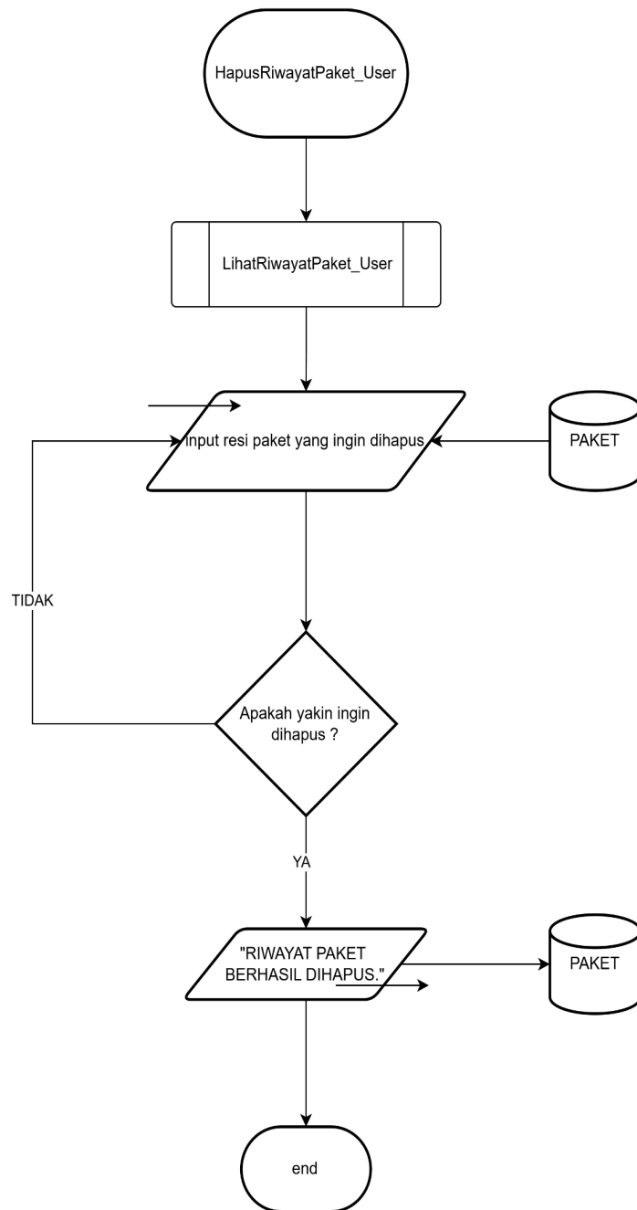
Gambar 9.1 Flowchart Hapus Riwayat Paket User
