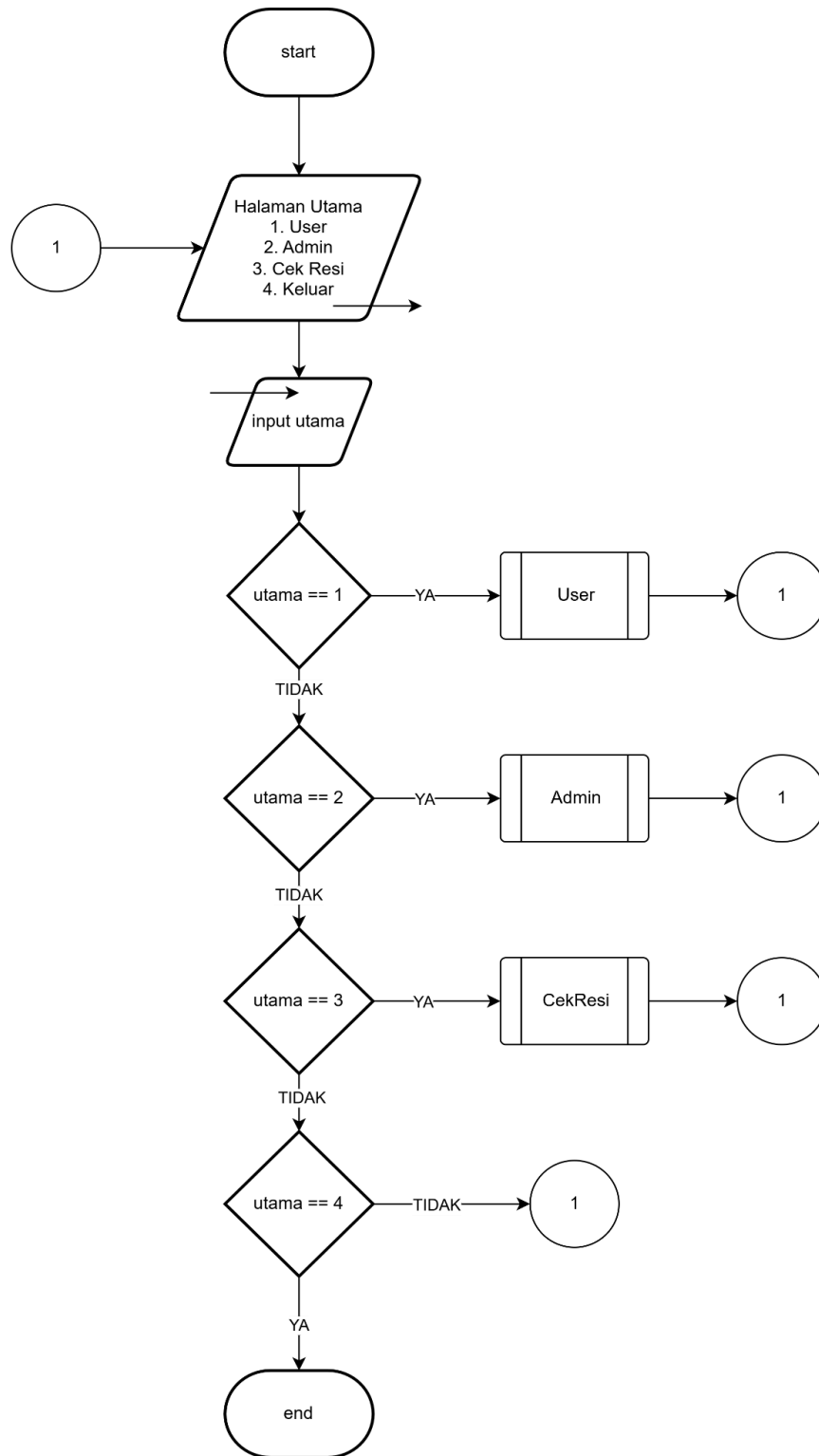
Gambar 1.1 Flowchart Main
