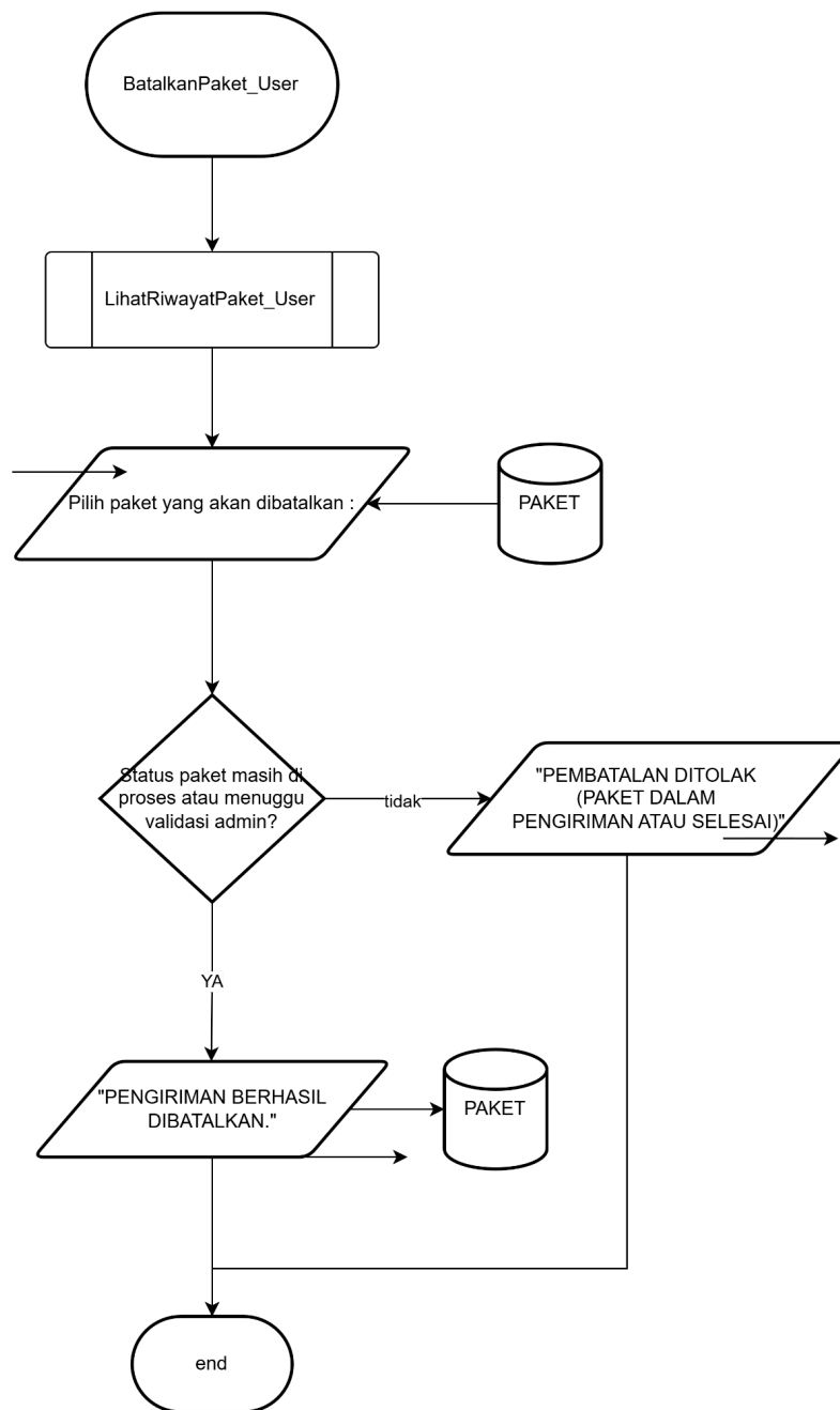
Gambar 10.1 Flowchart Batalkan Paket User
