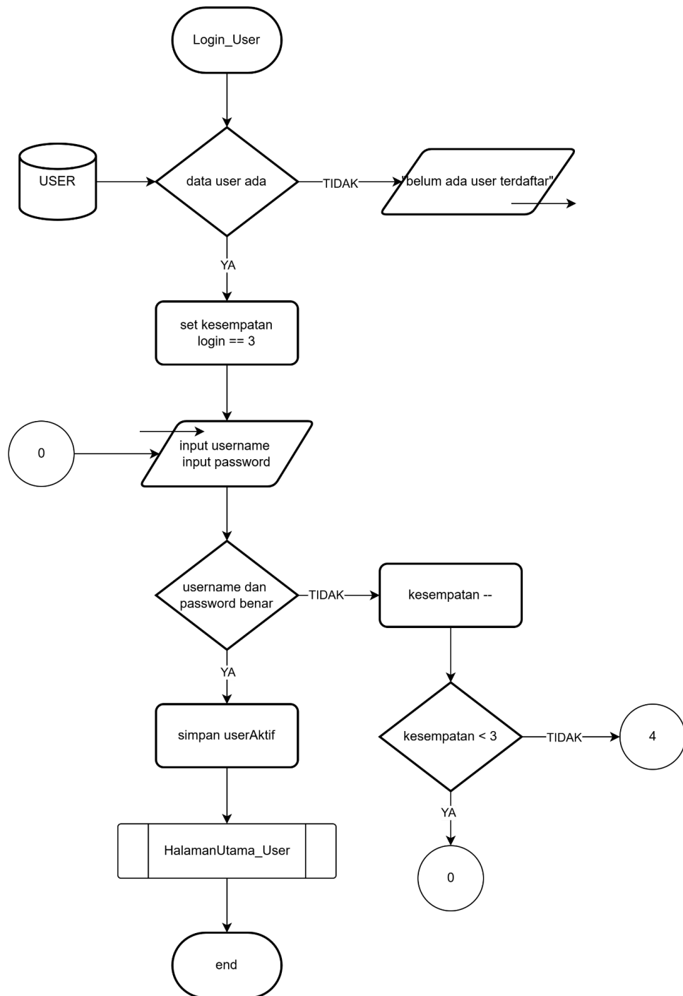
Gambar 4.1 Flowchart Login User
