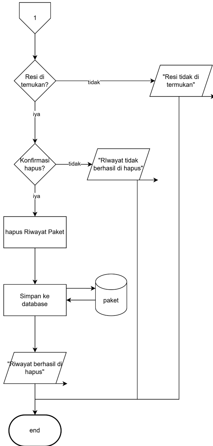
Gambar 16.1 Flowchart Hapus Riwayat Paket Admin (2)
