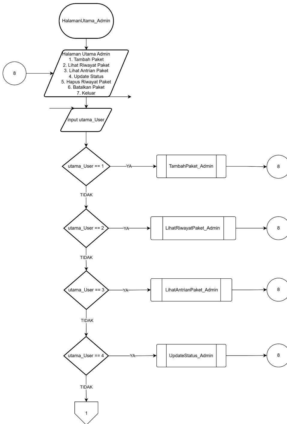
Gambar 12.1 Flowchart Halaman Utama Admin (1)
