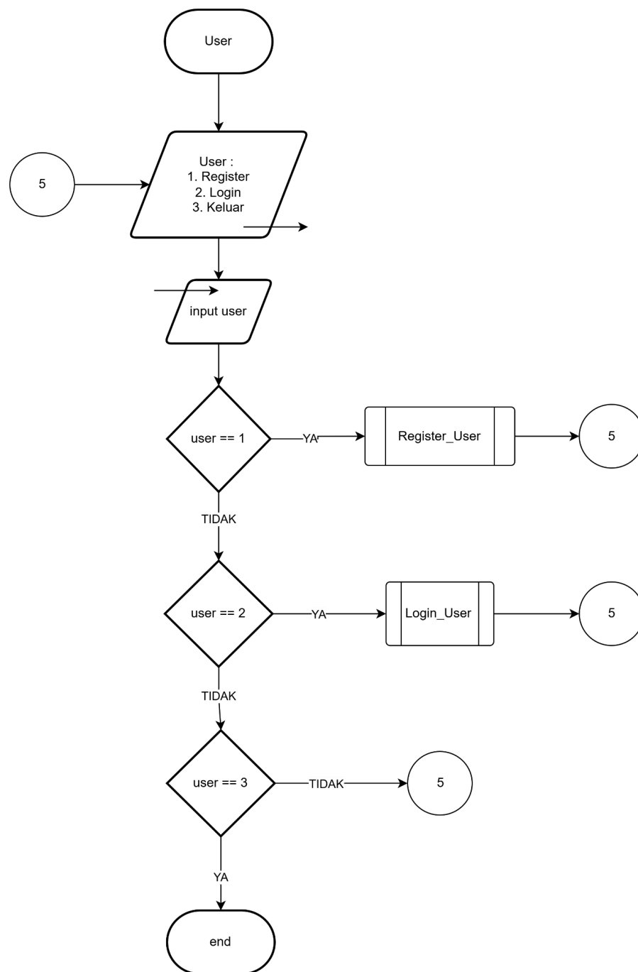
Gambar 2.1 Flowchart Menu User
